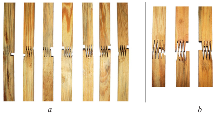
Fig. 5. The failure modes of the treated samples: a – glue failure; b – finger break failure
